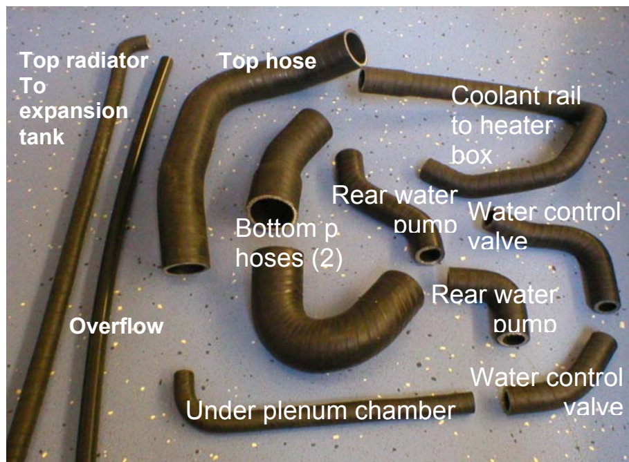
RV8 hose kit – set of eleven replacement hoses in silicone from Clive Wheatley
