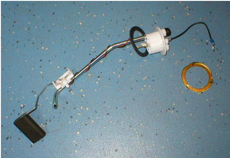
RV8 petrol tank sender unit with locking ring
