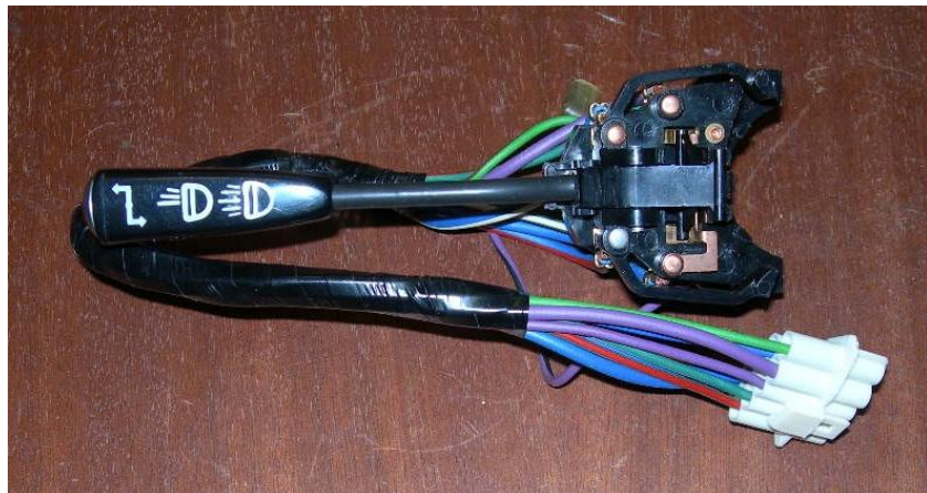
Indicator stalk
